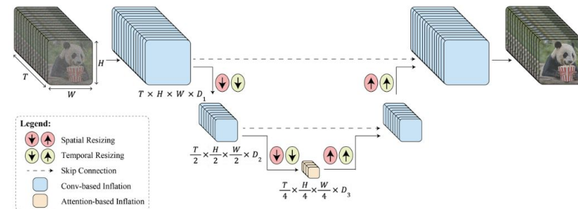
(a) Space-Time UNet (STUNet)
